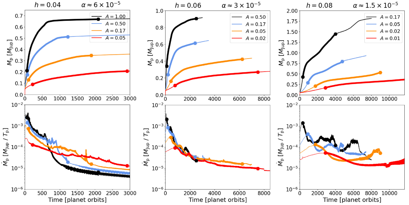
Figure 2. Planet mass (top panels) and planet mass accretion rate (bottom panels) as a function of time for cases with the lower viscosity \nu = 10^{-7} . A circle denotes the start of the vortex lifetime; a hexagon denotes the end. The vortex lifetime is highlighted in bold. The start and end of the vortex lifetime are marked on each side of the bold line with a circle and a hexagon, respectively. We measure the accretion rates as the increase in planet mass over each orbit divided by one orbit.
